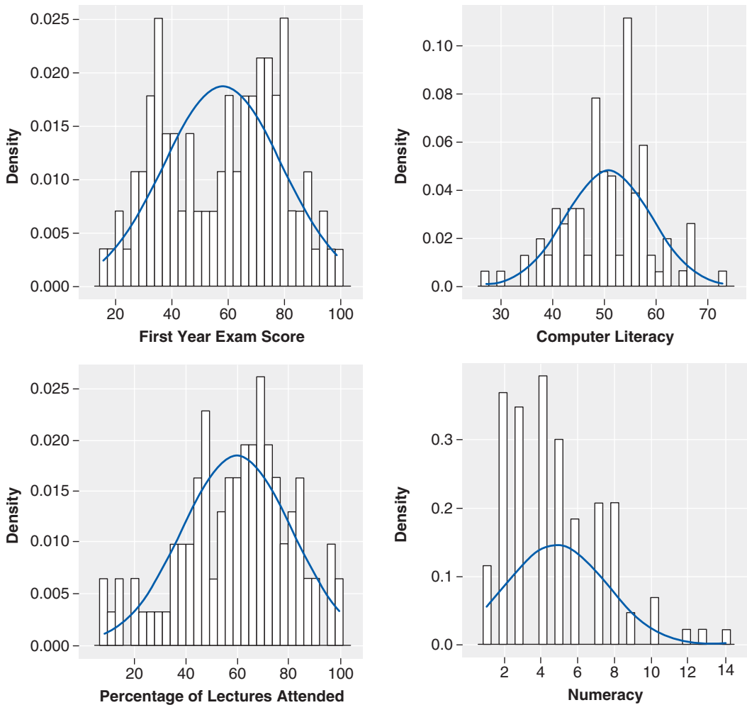
FIGURE 5.3 Histograms of the R exam data
